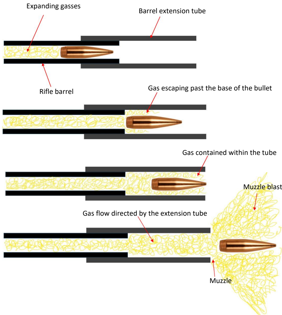
Pic 15 Showing how the barrel contains expanding gasses until they reach the muzzle (the end of the barrel) and can escape.
