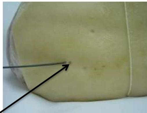
.177BB (steel) Impact velocity: 274 FPS (186 MPH) Impact energy: 1.20 joules Pellet weight: 5.3 grains Result: Skin breakage (no penetration)
