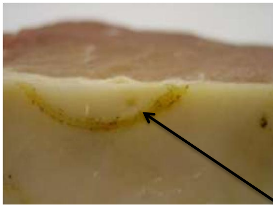
.177BB (steel) Impact velocity: 274 FPS (186 MPH) Impact energy: 1.20 joules Pellet weight: 5.3 grains Result: Skin breakage (no penetration)
